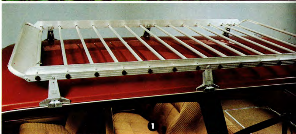
1. Estate Roof Rack 245/265. Made of aluminium it is light (just over 25 lbs) and strong (capacity 220 lbs). The 80" x 46" load platform is fitted with a spoiler to minimise noise and wind resistance. (1129660-5).
